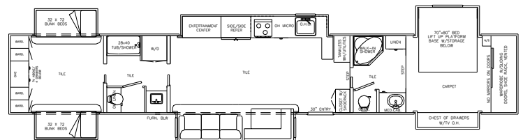
50' MARATHON FIFTH WHEEL 2 BATH/ 6 SLIDES
