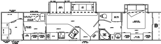
MARATHON 44 - 2 BEDROOM LS FIFTH WHEEL W/REAR OFFICE
